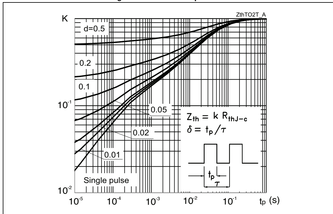
Figure 21. Thermal impedance
