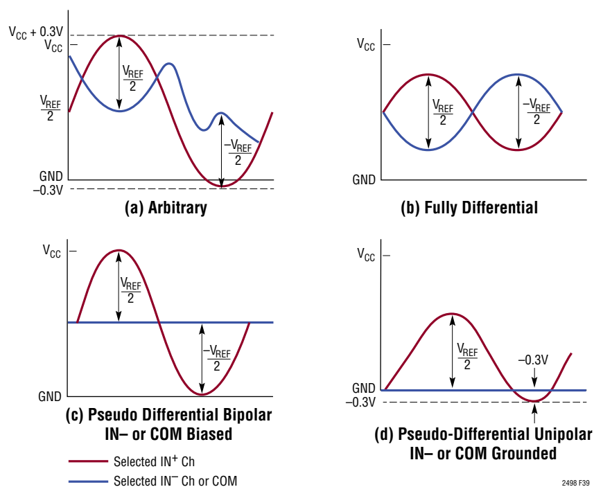
Figure 39. Input Range
