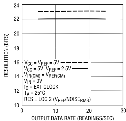
Figure 37. Resolution ( \text{Noise}_{RMS} \leq 1\text{LSB} ) vs Output Data Rate and Reference Voltage
