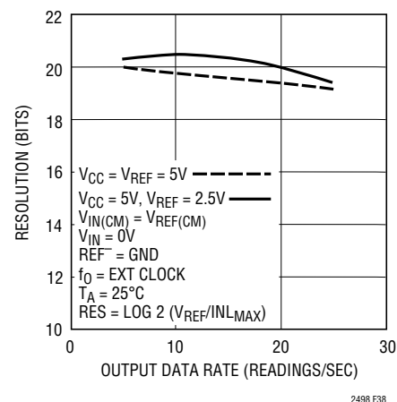
Figure 38. Resolution ( \text{INL}_{MAX} \leq 1\text{LSB} ) vs Output Data Rate and Reference Voltage
