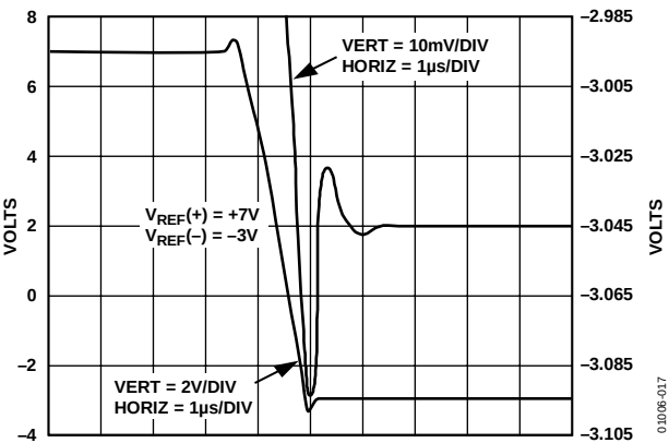
Figure 17. Settling Time(-)
