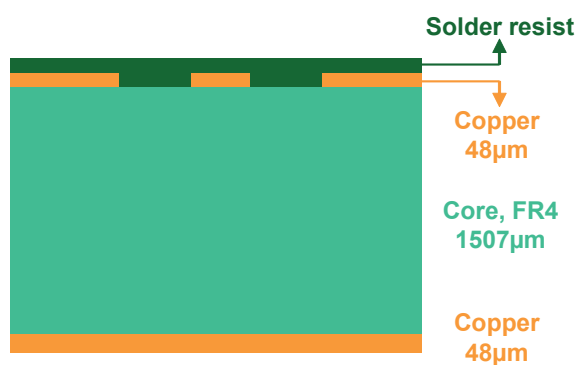
Figure 14. PCB stack-up recommendations
