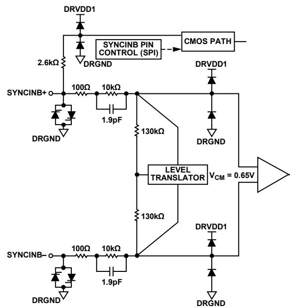
Figure 45. SYNCINB± Inputs
