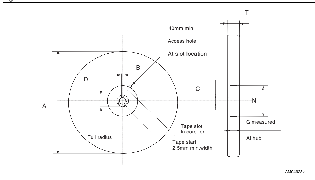
Figure 19. Reel schematic
