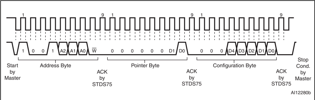
Figure 13. Configuration register WRITE
