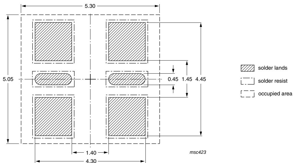
Fig 17. Reflow soldering footprint SOT457 (SC-74)
