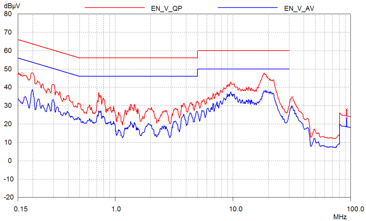
Figure 46 – Earth Ground at 230 VAC, Neutral.
