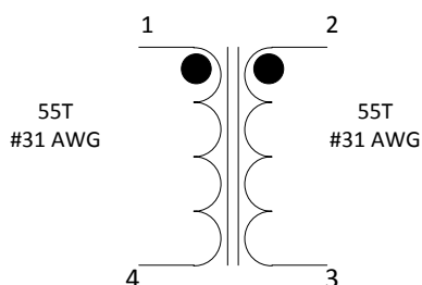
Figure 8 – Inductor Electrical Diagram.
