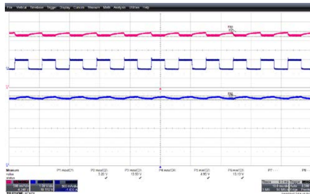
Figure 21 – 0.0 A – 0.5 A, 5 V Load Step Transient Response, 484 VAC. 5 V MIN : 4.95 V. 5 V MAX : 5.20 V. 12 V MIN : 13.13 V. 12 V MAX : 13.53 V. Upper: 5 V OUT , 0.5 V / div. Middle: 5 V Load, 0.5 A, 10 ms / div. Lower: 12 V OUT , 1 V / div.
