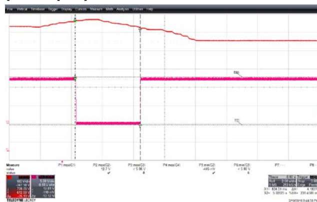
Figure 43 – Line Overvoltage.
