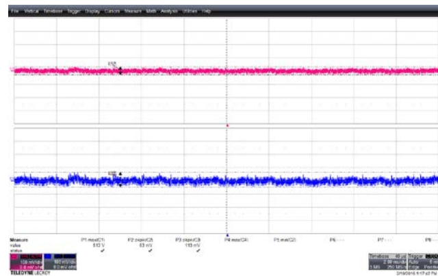
Figure 41 – Output Voltage Ripple Waveforms. 484 VAC Input. 1.25 A on 12 V. 5 V_{PK} : 63 mV, 12 V_{PK} : 113 mV. Upper: 5 V, 100 mV / div. Lower: 12 V, 100 mV, 2 ms / div..
