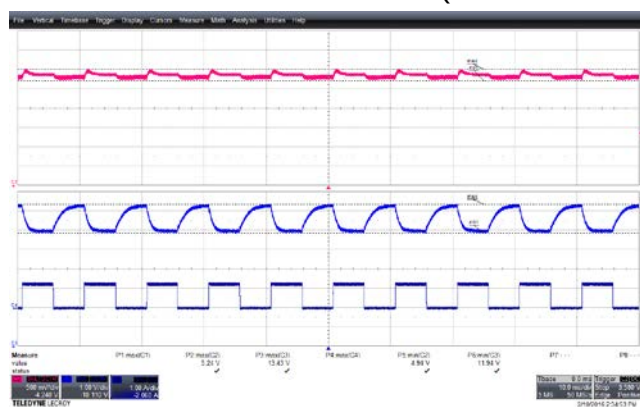
Figure 26 – 0.0 A – 1.25 A, 12 V Load Step Transient Response, 85 VAC.
