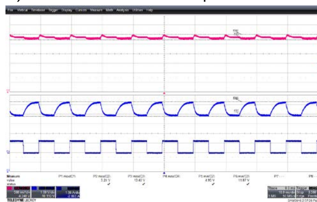
Figure 27 – 0.0 A – 1.25 A, 12 V Load Step Transient Response, 484 VAC.
