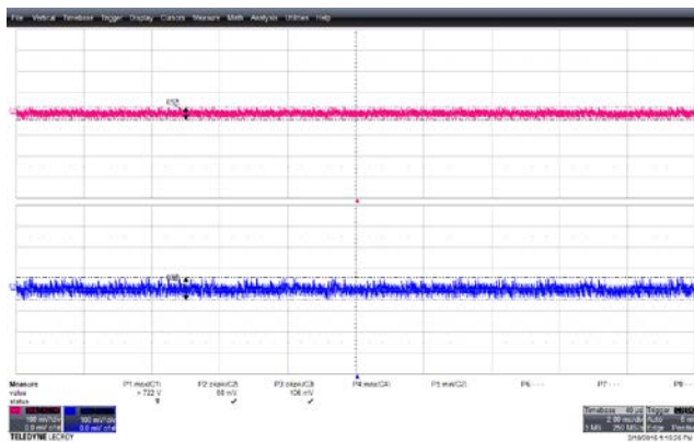
Figure 40 – Output Voltage Ripple Waveforms. 440 VAC Input. 1.25 A on 12 V. 5 V_{PK} : 60 mV, 12 V_{PK} : 106 mV. Upper: 5 V, 100 mV / div. Lower: 12 V, 100 mV, 2 ms / div.
