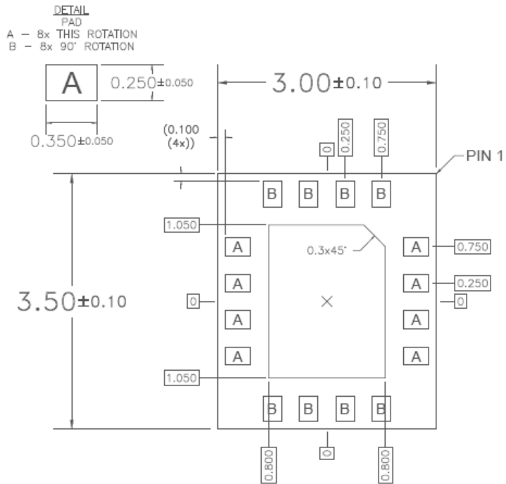
BOTTOM VIEW
