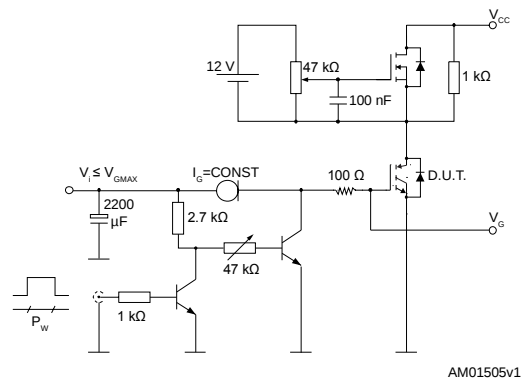
Figure 29: Gate charge test circuit
