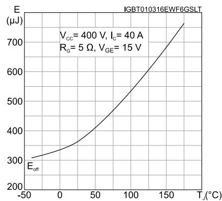
Figure 18: Switching energy vs temperature
