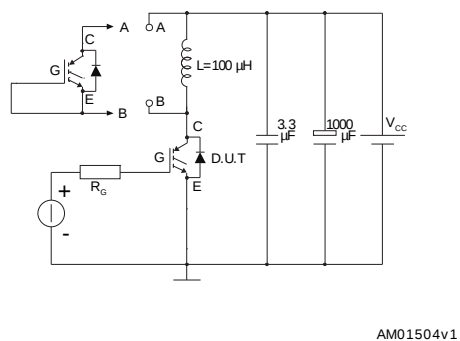
Figure 28: Test circuit for inductive load switching
