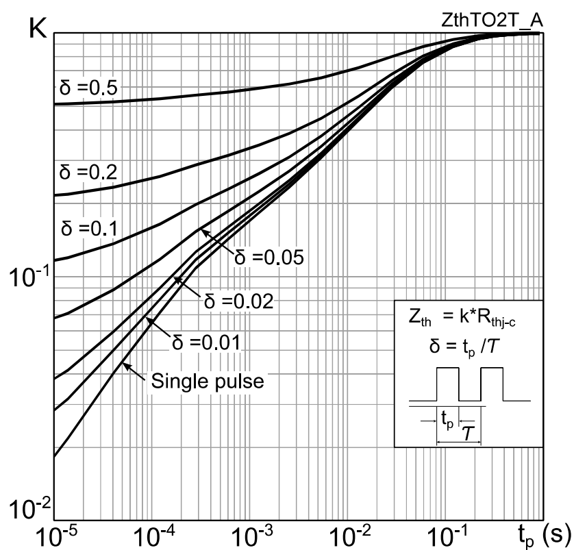
Figure 26: Thermal impedance
