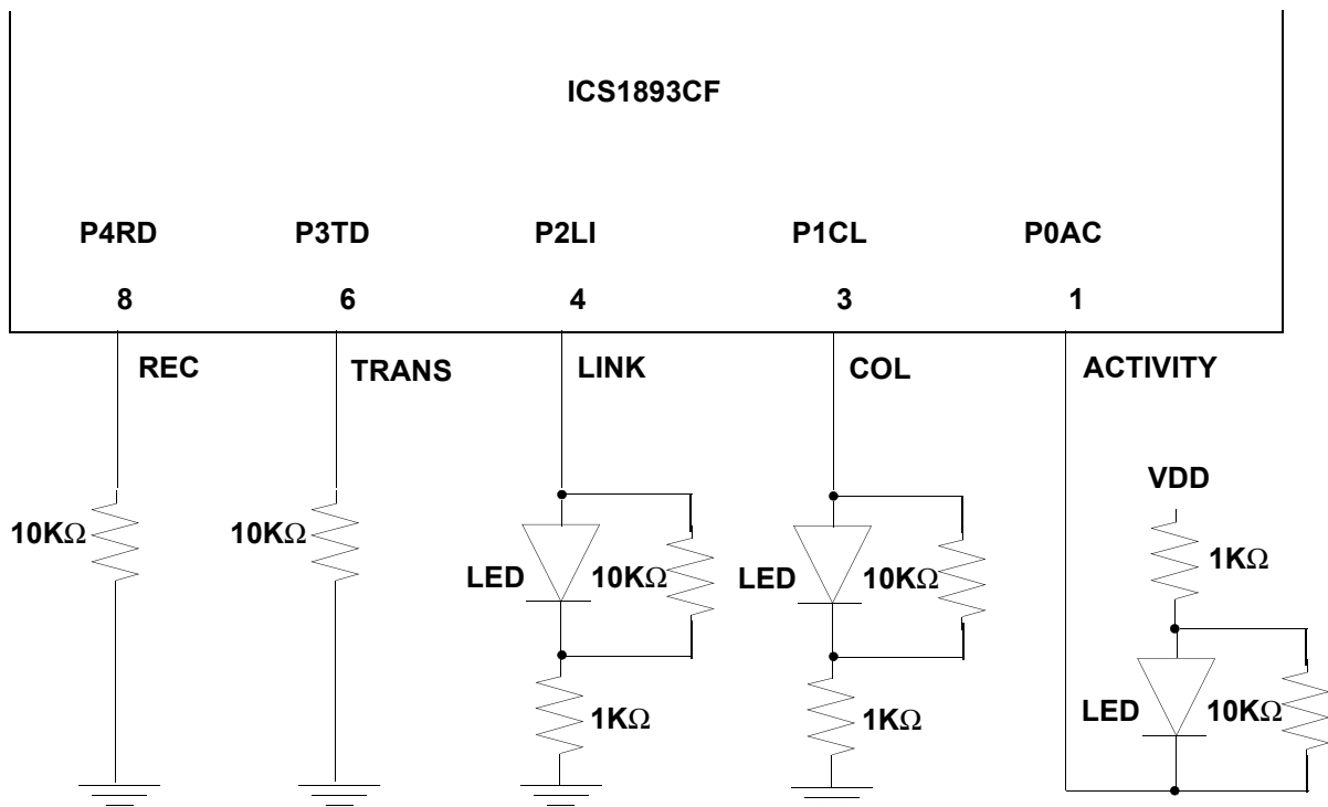
Figure 5-3. ICS1893CF LED - PHY Interface
