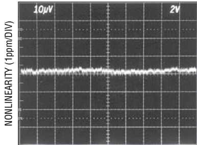
Gain Nonlinearity, G = 1
