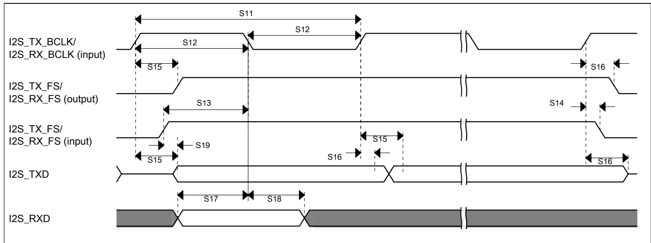
Figure 45. I2S/SAI timing — slave modes
