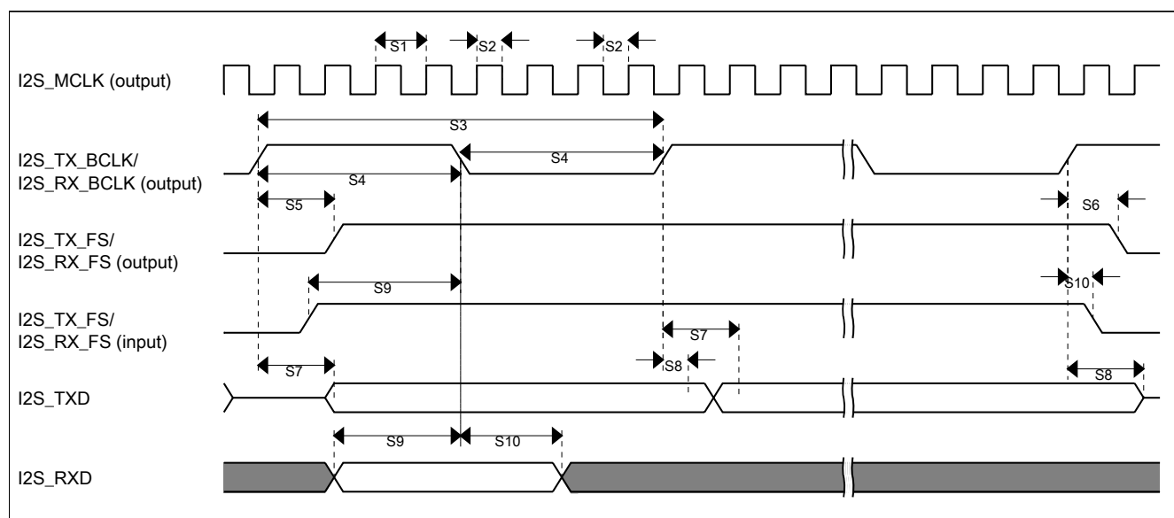
Figure 42. I2S/SAI timing — master modes
