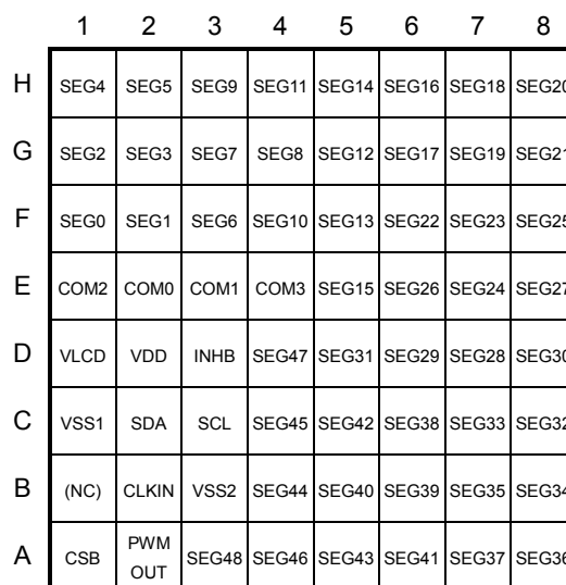
Figure 7. Pin Configuration (TOP VIEW)
