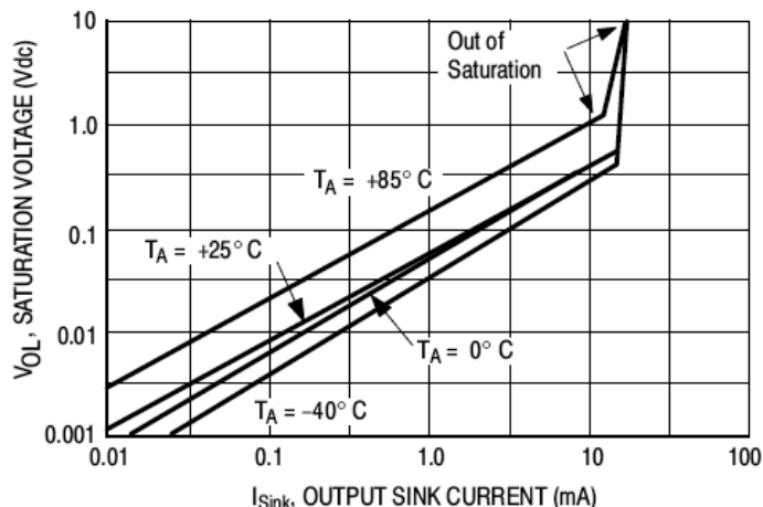
Figure 2. Output Saturation Voltage vs. Output Sink Current
