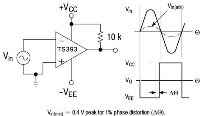
Figure 6. Time Delay Generator
