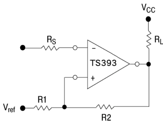
Figure 8. Comparator with Hysteresis
