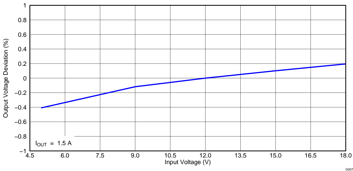
Figure 8. TPS54394EVM Converter 2 Line Regulation
