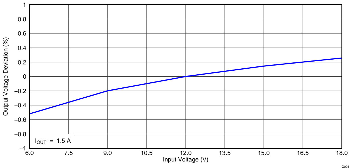
Figure 7. TPS54394EVM Converter 1 Line Regulation
