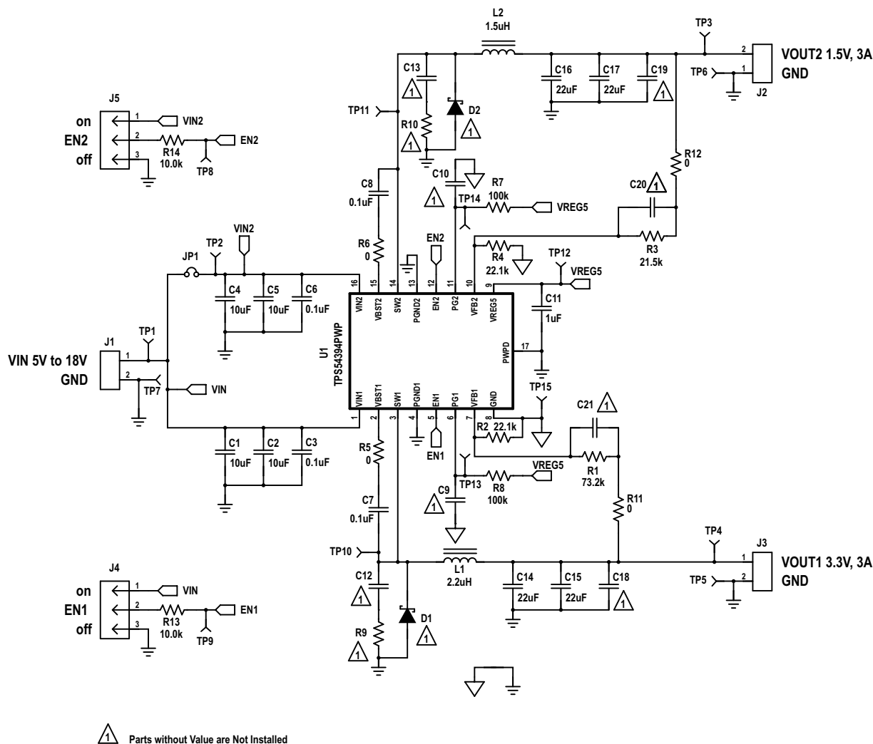
Figure 26. TPS54394EVM Schematic Diagram
