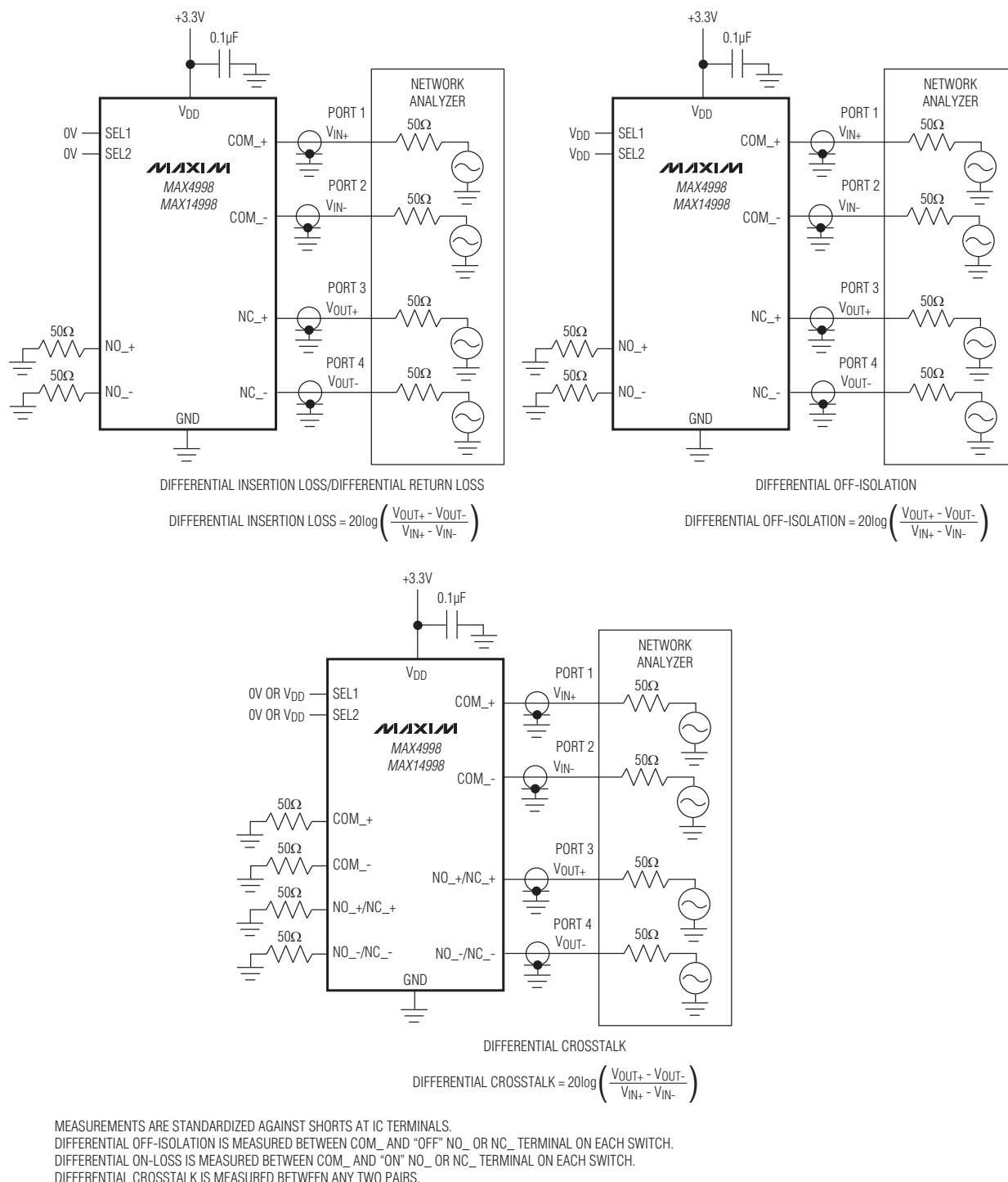
Figure 2. Differential On-Loss, Differential Off-Isolation, and Differential Crosstalk
