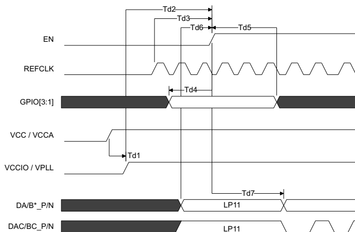
Figure 1. Power-Up Timing Definitions for DPPLL_CLK_SRC = REFCLK
