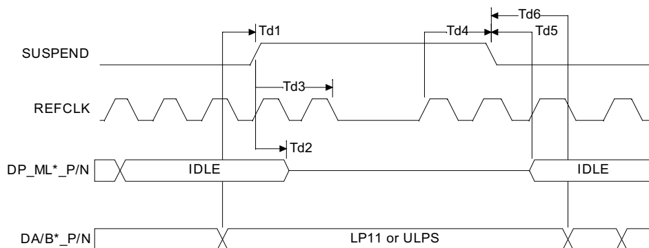
Figure 5. SUSPEND Timing Definitions
