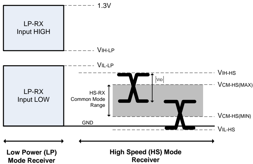
Figure 4. DSI Receiver Voltage Definitions
