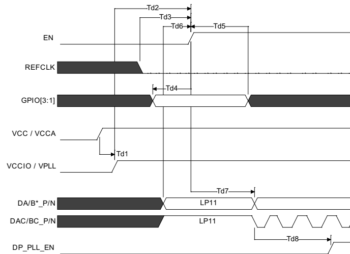
Figure 2. Power-Up Timing Definitions for DPPLL_CLK_SRC = DACP/N
