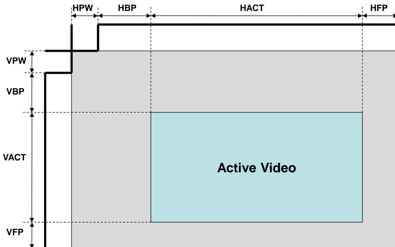
Figure 16. Video Format
