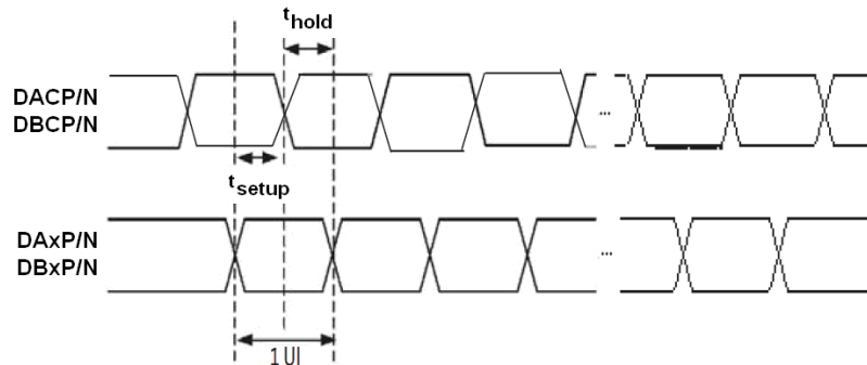
Figure 3. DSI HS Mode Receiver Timing Definitions
