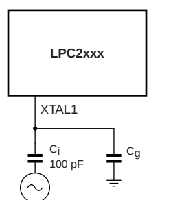
Fig 22. Slave mode operation of the on-chip oscillator
