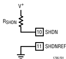
Figure 1. R_{\text{SHDN}} Connected Between V^+ and SHDN (Pin 10); SHDNREF (Pin 11) = GND. See Figure 2
