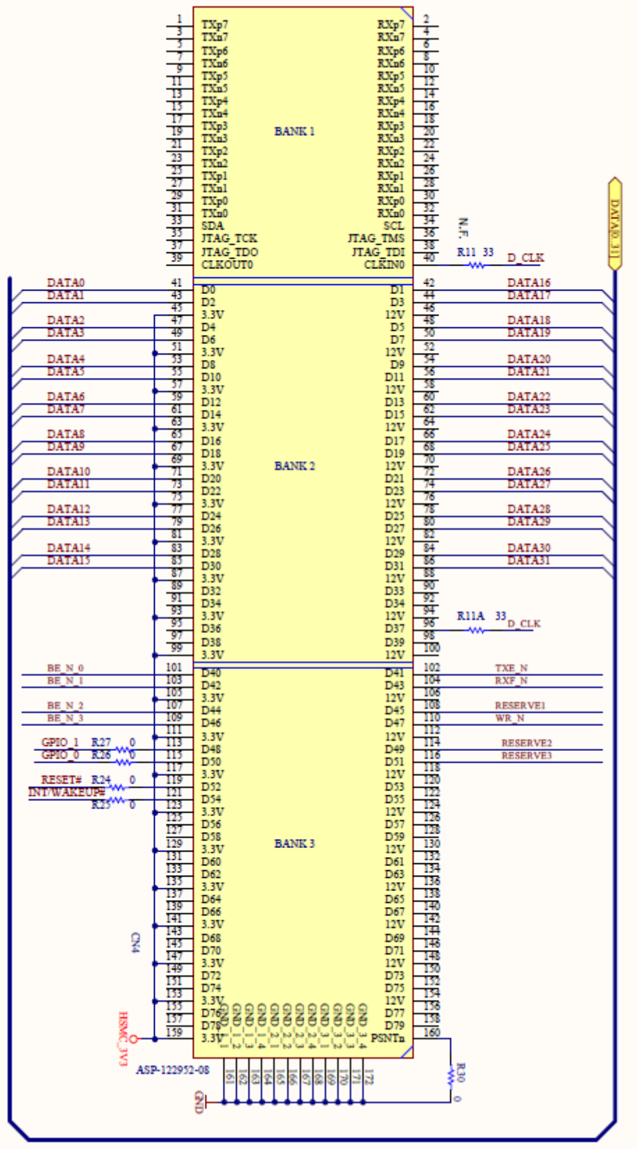
Figure 3-3 Schematics: HSMC_UMFT602A
