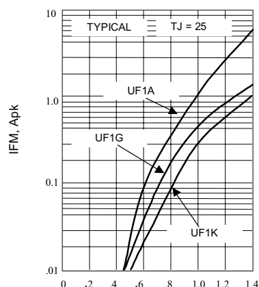
Fig. 2-FORWARD CHARACTERISTICS
