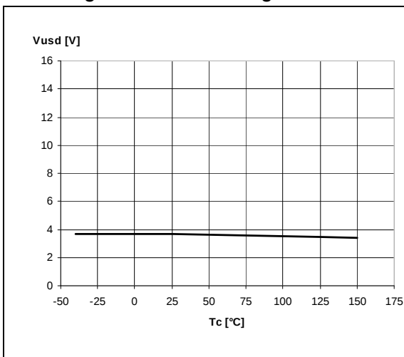
Figure 27. Turn-on voltage slope
