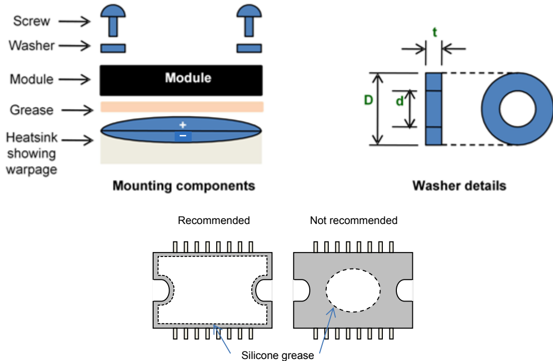
Figure 16. Module Mounting details: components; washer drawing; need for even spreading of thermal grease
