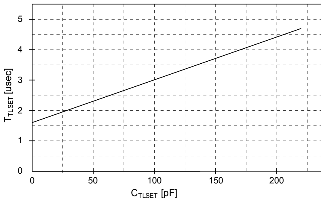
Figure 7-10 Typical T_{TLSET} Time over C_{TLSET} Capacitance
