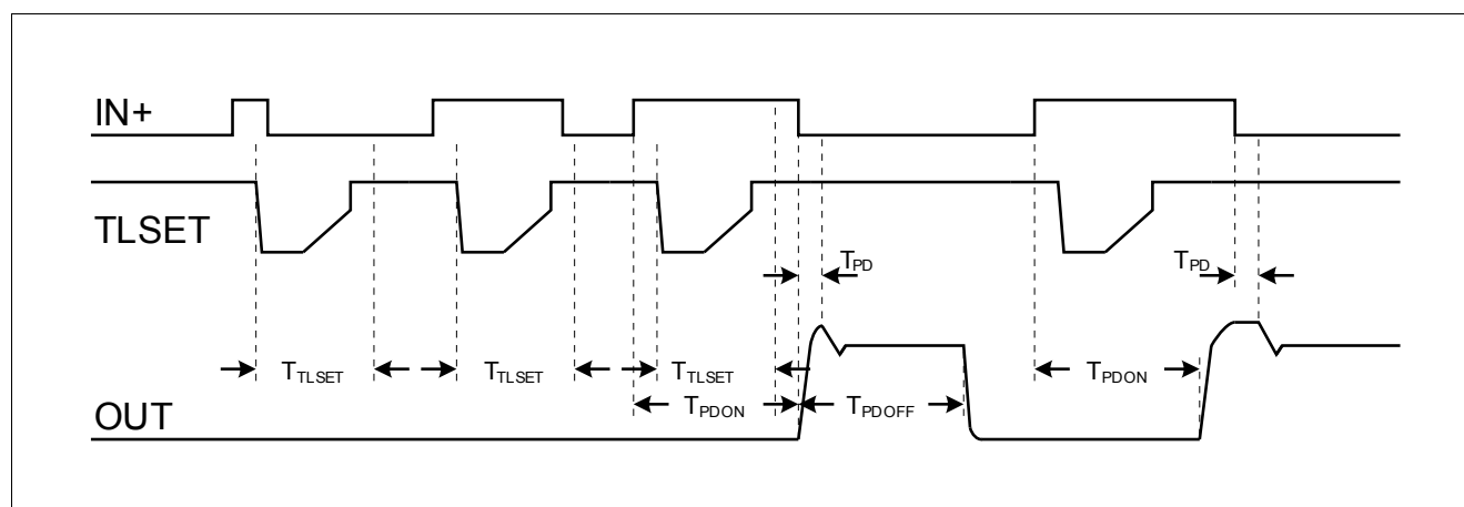
Figure 7-5 Short Switch ON Pulses
