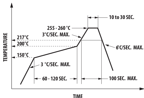
Figure 20: Recommended Lead-Free Reflow Soldering Condition
