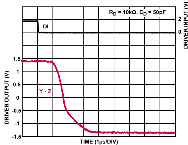
FIGURE 13. ISL32614E DRIVER WAVEFORMS, HIGH-TO-LOW
