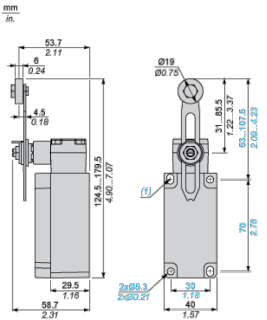
(1) 2 elongated holes 5.3 x 7.3 mm / 0.21 x 0.29 in.
