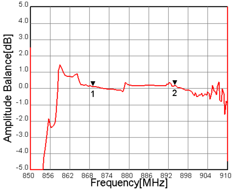
Fig.7 Amplitude Balance
