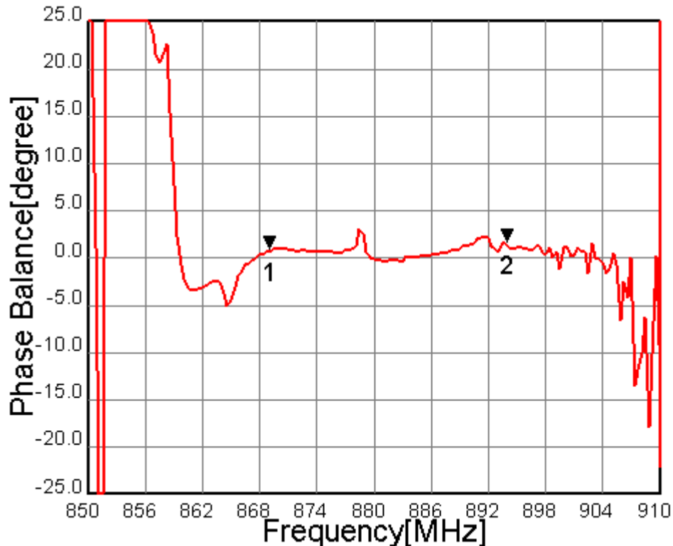
Fig.8 Phase Balance
