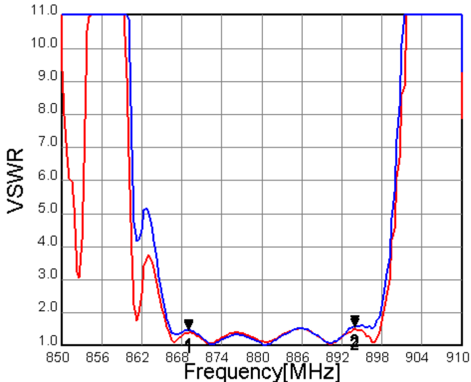
Fig.2 VSWR
