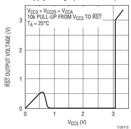
\overline{RST} Output Voltage vs Supply Voltage (LTC1726-2.5)
