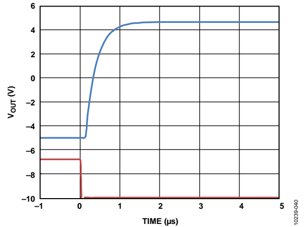
Figure 39. Rising Full-Scale Voltage Step
