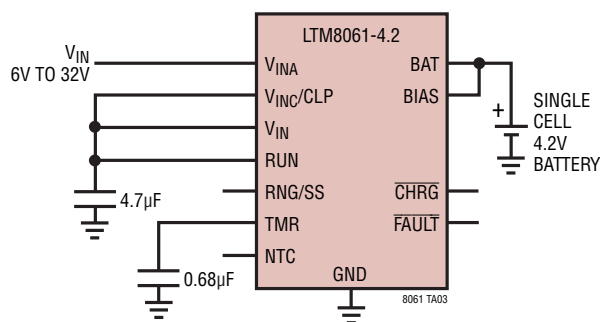
Single Cell 2A Li-Ion Battery Charger with 3 Hour Timer Termination and Reverse Input Protection
