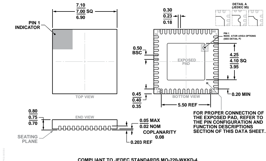
Figure 31. 48-Lead Lead Frame Chip Scale Package [LFCSP] 7 mm × 7 mm Body and 0.75 mm Package Height (CP-48-5)
