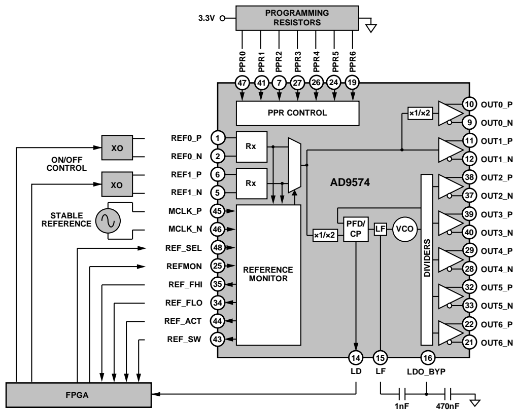
Figure 24. Dual Oscillator Reference Input Application Diagram
