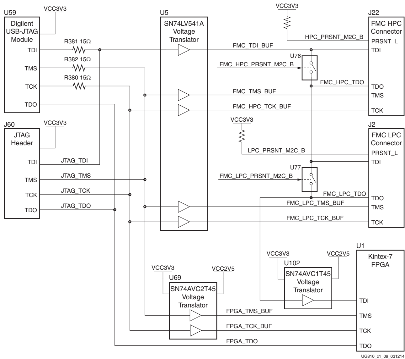
Figure 1-9: JTAG Circuit
