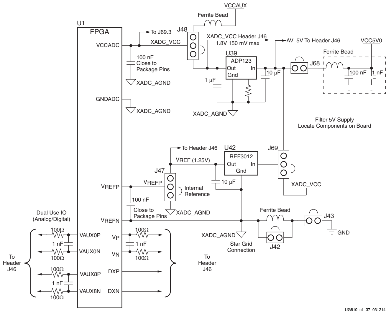
Figure 1-36: Header XADC_VREF Voltage Source Options
