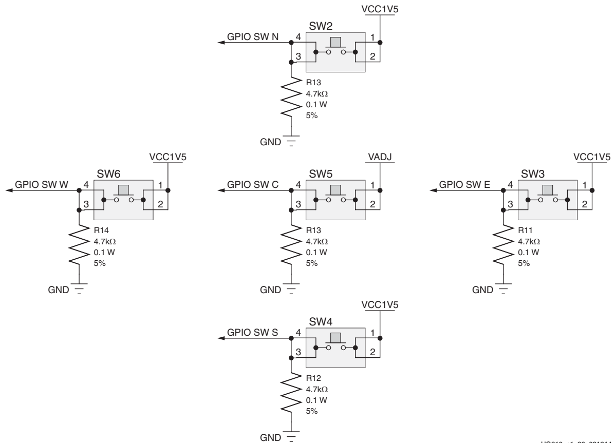
Figure 1-25: User Pushbuttons
