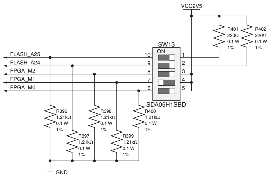
Figure 1-38: Mode Switch
