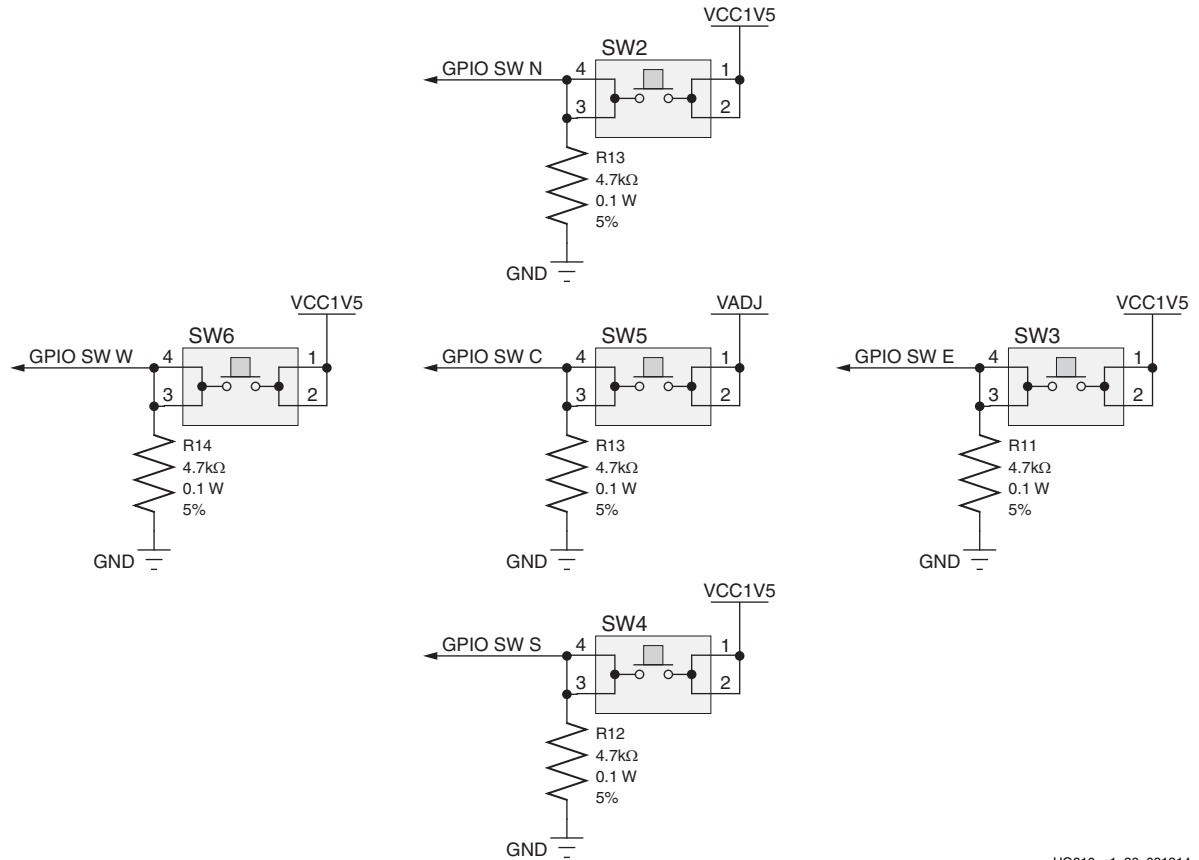
Figure 1-25: User Pushbuttons
