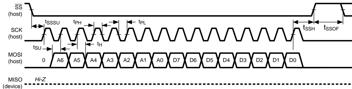
Figure 2. SPI Write
