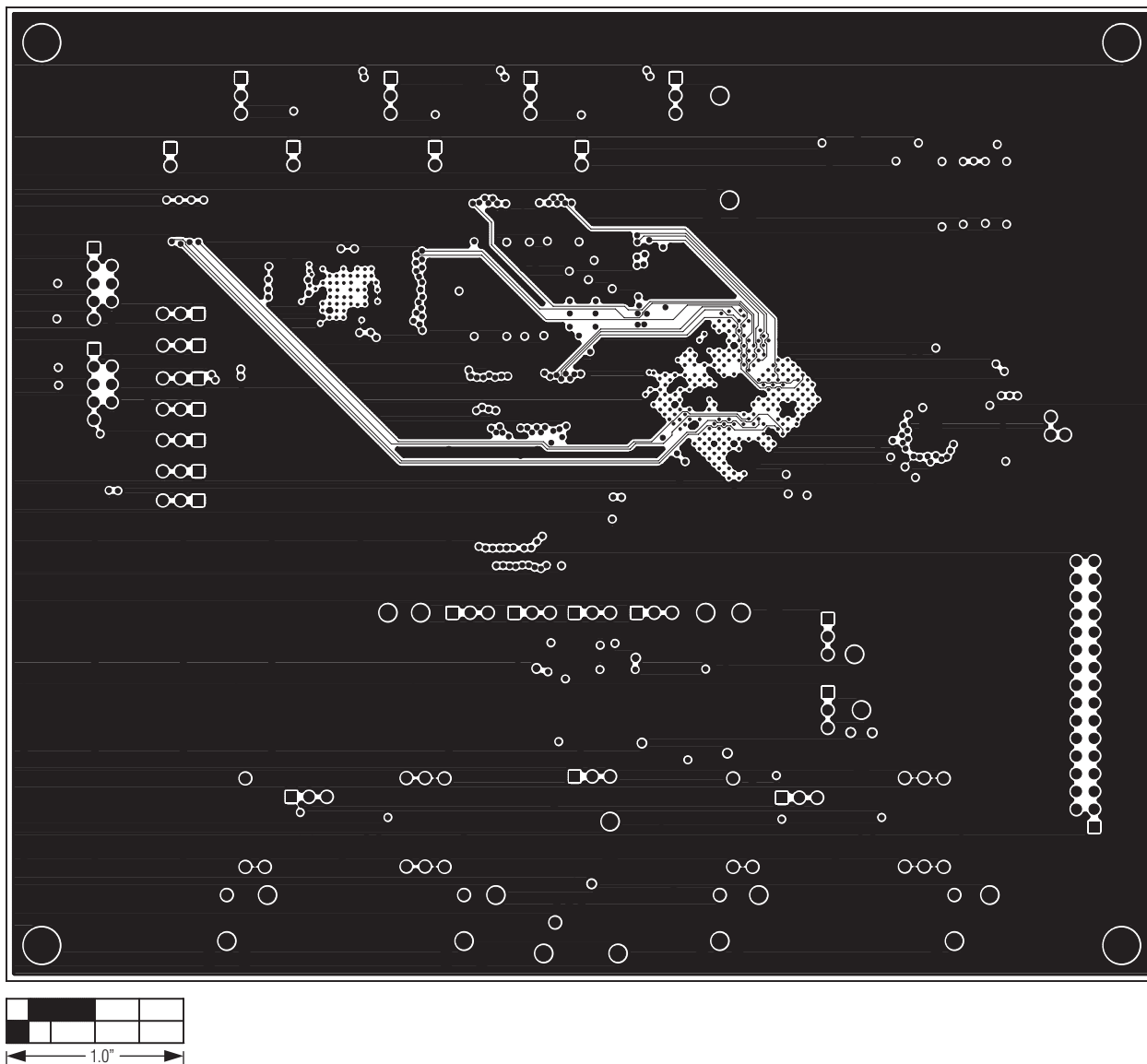
Figure 16. MAX11666 EV Kit PCB Layout—Layer 9
