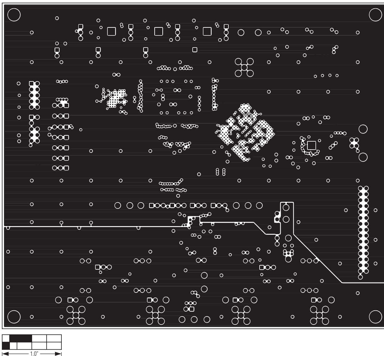
Figure 18. MAX11666 EV Kit PCB Layout—Layer 11
