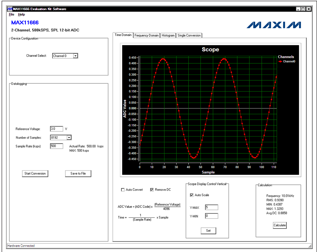
Figure 2b. Time Domain Tab (Zoomed In)
