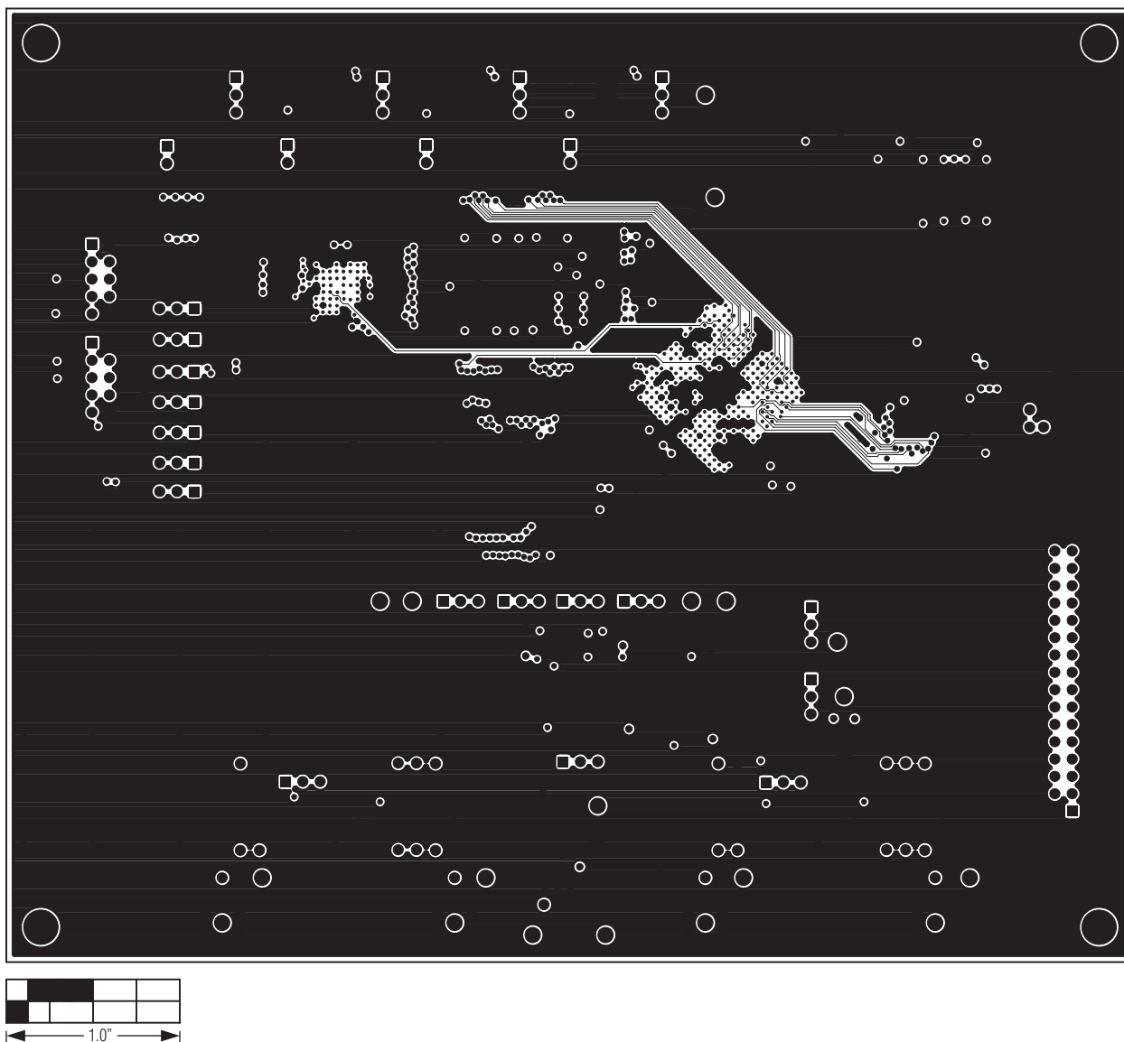
Figure 14. MAX11666 EV Kit PCB Layout—Layer 7
