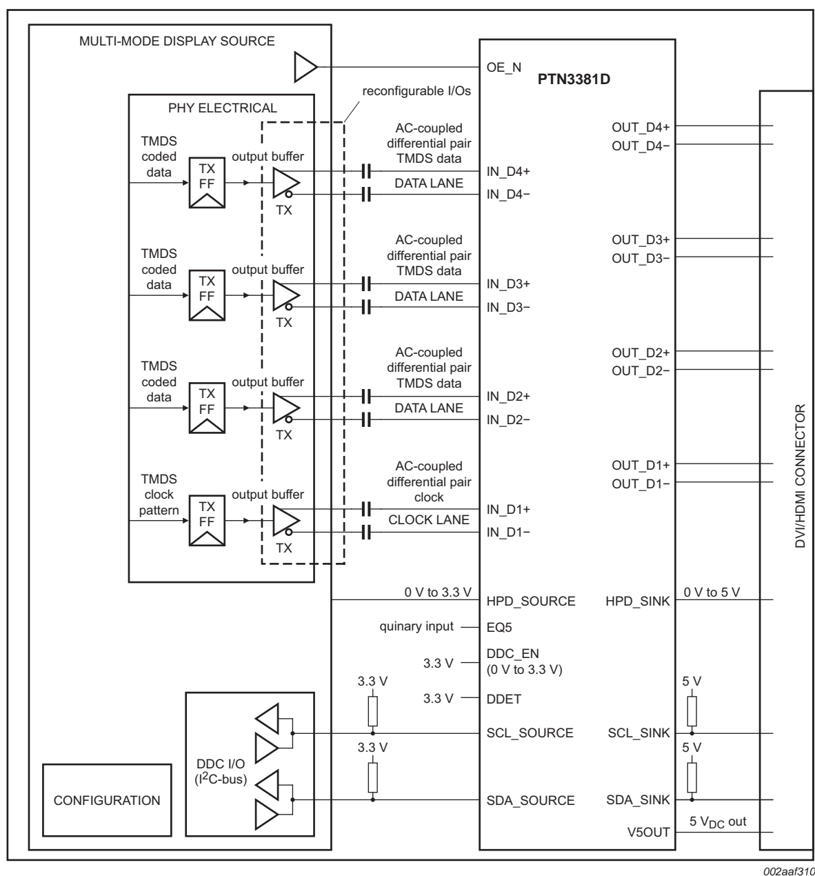
Fig 1. Typical application system diagram
