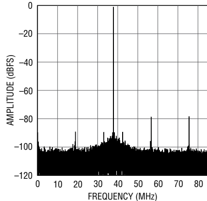
LTC2150-12: 32K Point FFT, f_{IN} = 380\text{MHz} , -1\text{dBFS} , 170Msps
