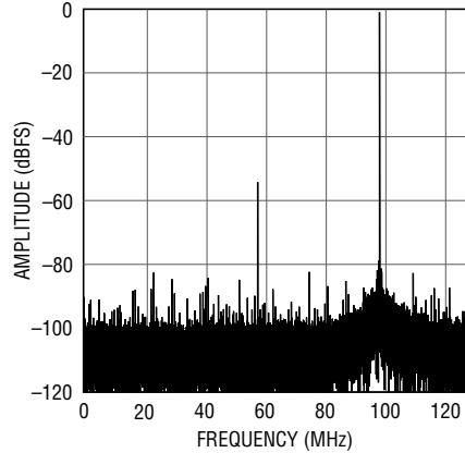
LTC2152-12: 32K Point FFT, f_{IN} = 907\text{MHz} , -1\text{dBFS} , 250Mps
