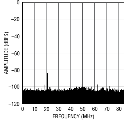
LTC2150-12: 32K Point FFT, f_{IN} = 121\text{MHz} , -1\text{dBFS} , 170Msps
