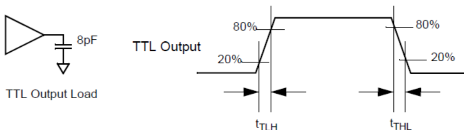
Figure 6. CLKIN Transmission Time
