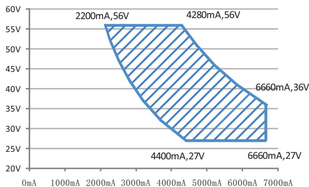
◎ XLG-240-H
