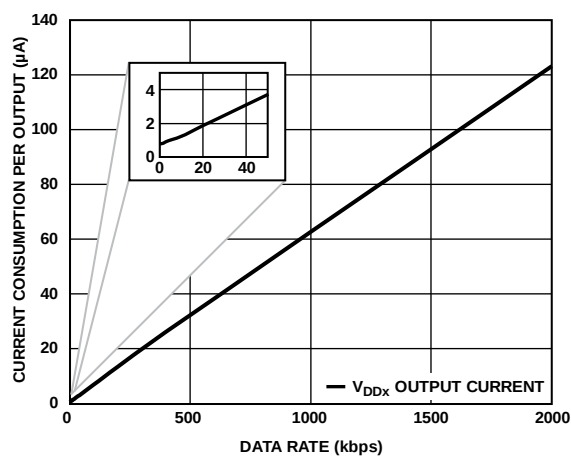
Figure 14. Current Consumption per Output vs. Data Rate for 3.3 V, EN_x = Low Operation
