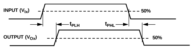
Figure 31. Propagation Delay Parameters
