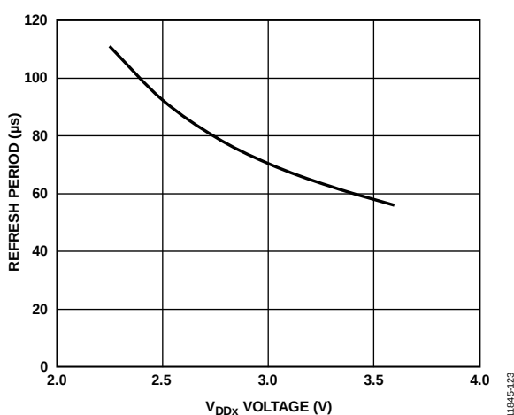
Figure 28. Typical Refresh Period vs. V_{DDX} Voltage
