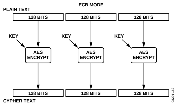
Figure 105. ECB Mode.
