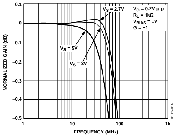
Figure 14. 0.1 dB Flatness
