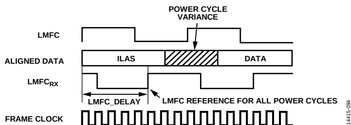
Figure 102. LMFC_DELAY_x to Compensate for Link Delay &gt; LMFC
