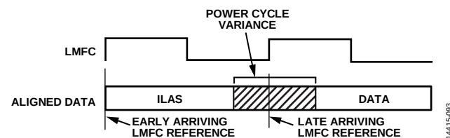
Figure 101. Link Delay &gt; LMFC Period Example
