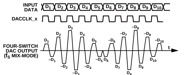
Figure 128. Mix-Mode Waveform
