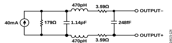
Figure 139. Equivalent Circuit Model of the DAC Output
