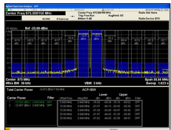
Figure 34. Two-Carrier W-CDMA at 875 MHz
