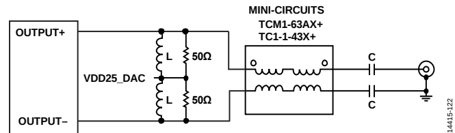
Figure 138. Recommended Transformer for Wideband Applications with Upper Bandwidths of up to 5 GHz
