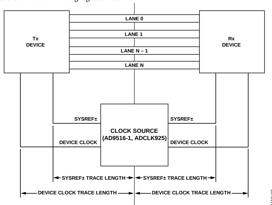
Figure 125. SYSREF \pm Signal and Device Clock Trace Length
