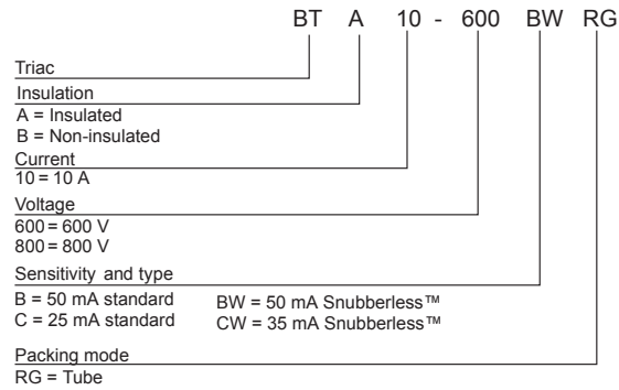
Figure 15. BTA10 and BTB10 series ordering information scheme
