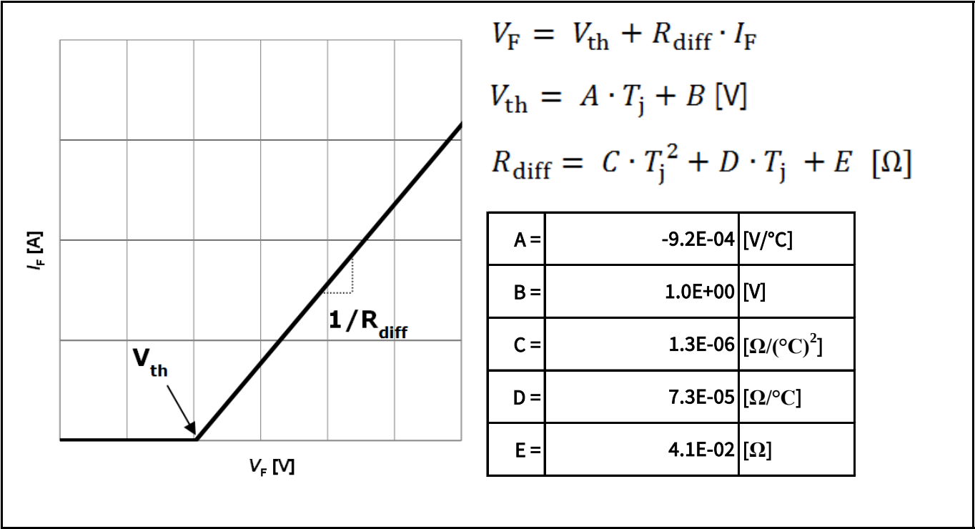
Figure 6 Simplified forward characteristics model V_F = f(I_F) ; -40^\circ\text{C} < T_j < 175^\circ\text{C} ; I_F < 20 A
